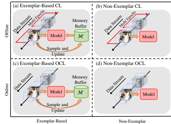
Figure 1: The comparison between (a) the Exemplar-Based CL, (b) the Non-Exemplar CL, (c) the Exemplar-Based OCL, and (d) the investigated Non-Exemplar OCL in this paper. In the last scenario, all data can only be learned for one epoch and none of them can be retained as exemplars for reusing.
