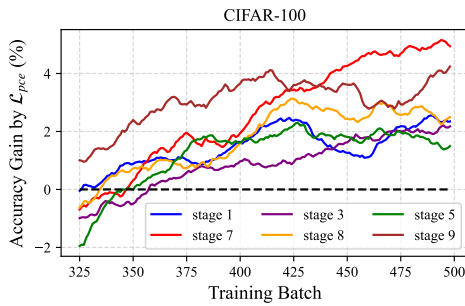
Figure 7: Accuracy gain of previously seen samples brought by \mathcal{L}_{pce} .
