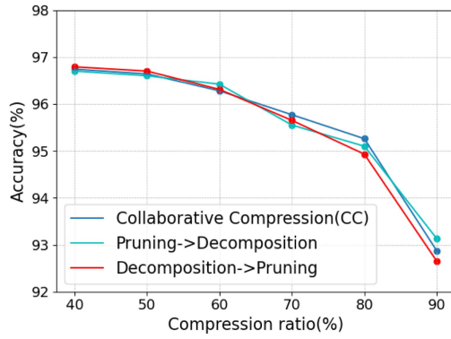
Fig. 8. Compression of different orders of CC on UCI-HAR.
