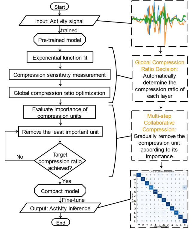
Fig. 2. Flow-chart of Collaborative Compression procedure.
