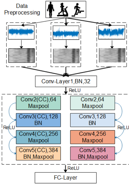
Fig. 5. Brief description for architecture.
