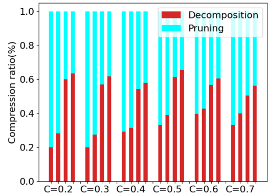
Fig. 10. Compression ratios of different compression operations in different layers of PAMAP2.
