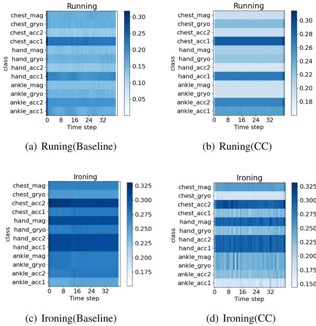
Fig. 11. The effectiveness of Collaborative Compression .
