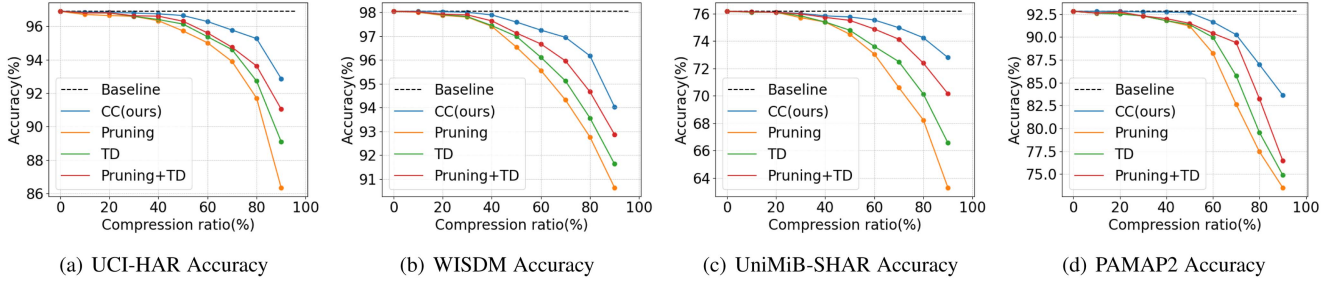
Fig. 4. Comparison of the accuracy under different compression ratios, TD means tensor decomposition.
