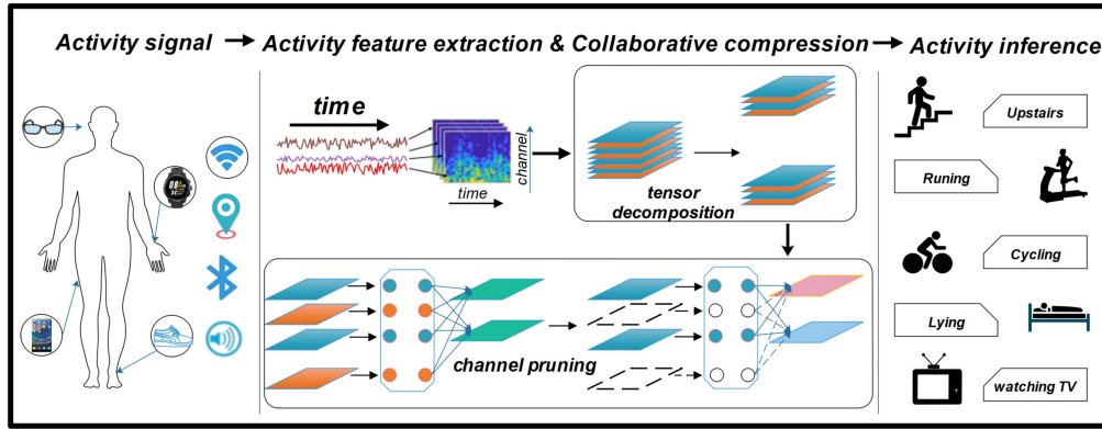
Fig. 1. The overview of the Collaborative Compression scheme.
