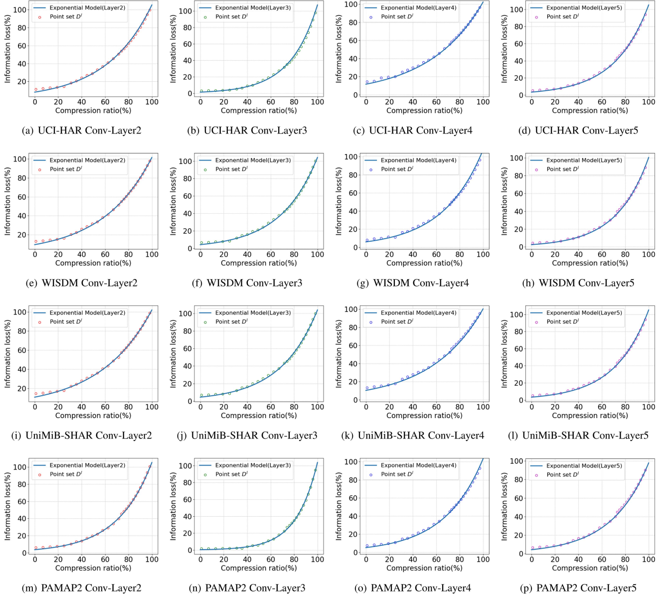
Fig. 3. Compression sensitivity analysis of different datasets.
