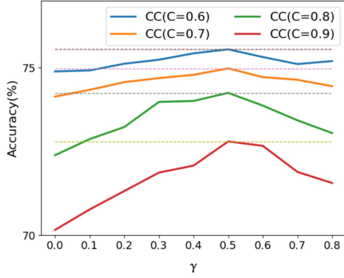
Fig. 7. Influence of different \gamma on UniMiB-SHAR.
