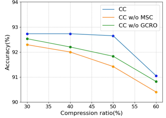
Fig. 6. Independent influence of Compression Ratio Optimization (GCRO) algorithm and Multi-Step Compression (MSC) on PAMAP2.
