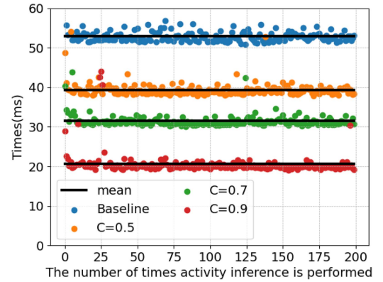
Fig. 13. Inference speed over 200 times.
